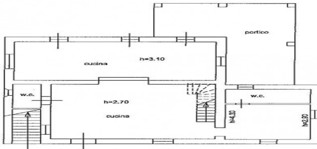
Piano Terra
